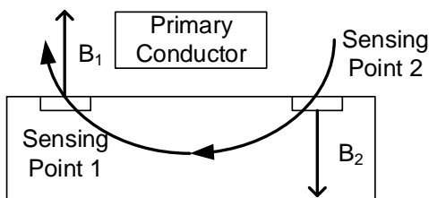
Figure 4: Cross Section of the Sensor
