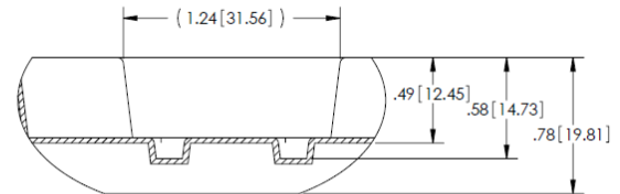
DETAIL C SCALE 2:1
