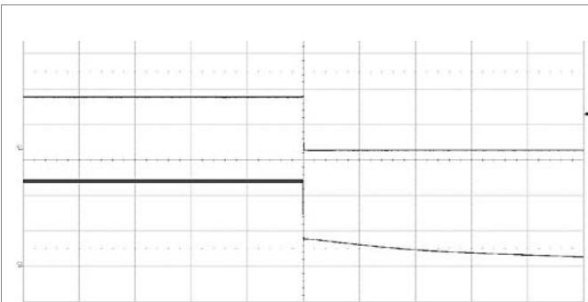
Output disabled by removing V_I at: T_{P1} = +25^\circ\text{C} , V_I = 24\text{ V} , I_O = 2\text{ A} resistive load. Top trace: output voltage (10 V/div.). Bottom trace: input voltage (10 V/div.). Time scale: (200 ms/div.).
