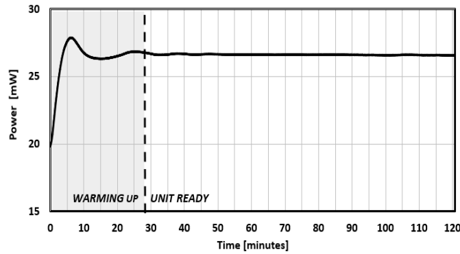
FIG. 11: WARM-UP TIME
